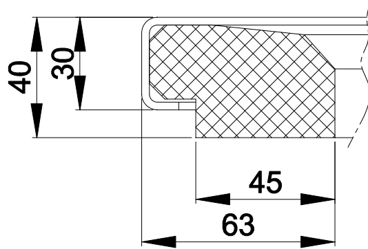
Detail A M5:1
