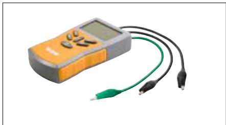
Schlüter®-DITRA-HEAT-E-CT kabeltester
