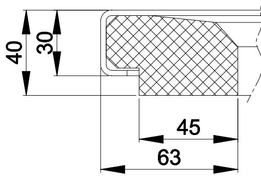
Detail A M5:1
