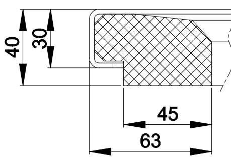
Detail A M5:1
